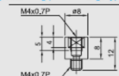
(3) FS nipple connector for side grease fitting (FL, FLL flange type only)
