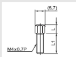
(1) Standard grease fitting (Front grease fitting)
